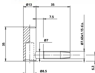
Cilindrična spojnica CF100150N007 / Hinge CF100150N007
